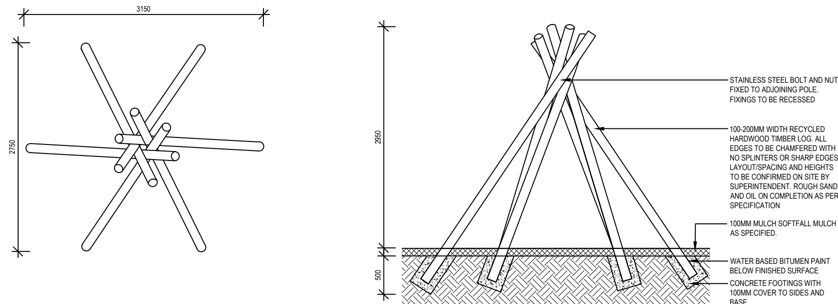
TEE PEE TYPICAL DETAIL SCALE NTS
