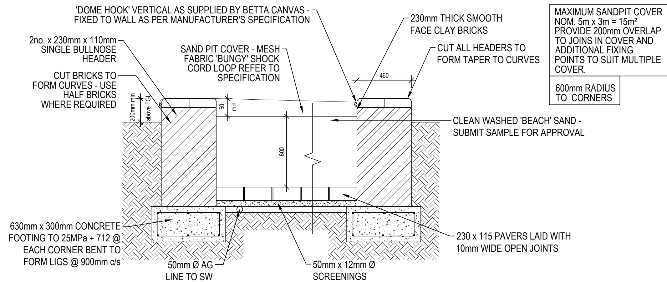
KINDERGARTEN/PRESCHOOL SAND PIT SECTION - TYPICAL FOR ALL SAND PITS SCALE 1:40 @ A3
