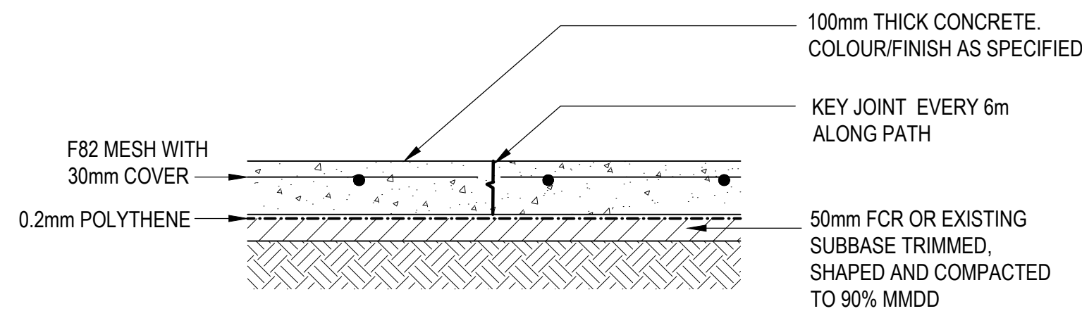
CONCRETE PATH DETAIL SCALE 1:20 @ A3
