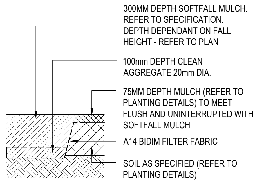
PLAYGROUND MULCH TO GARDEN BED SCALE 1:40 @A3
