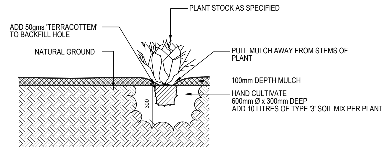
'SPOT' PLANTING DETAIL SCALE 1:20 @A3
