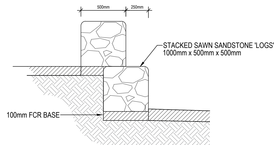
STACKED SANDSTONE 'LOGS' DETAIL SCALE 1:40 @ A3
