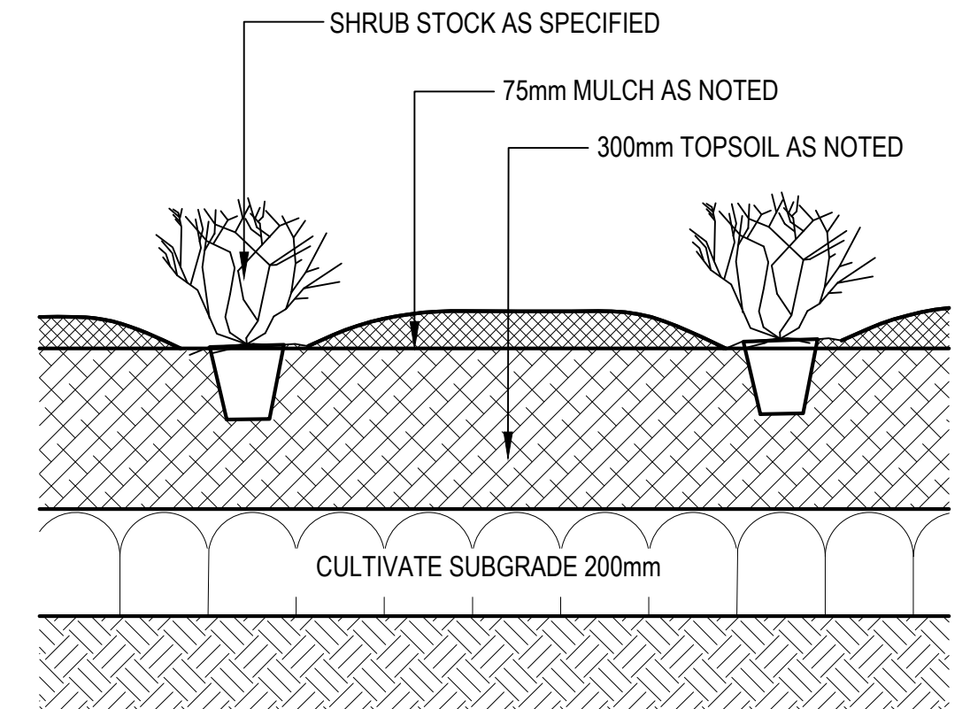
SHRUB PLANTING DETAIL SCALE 1:50 @ A3
