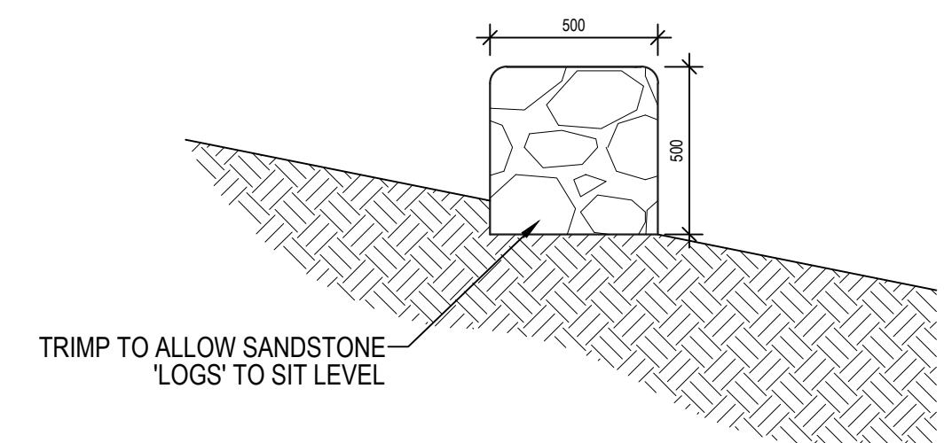
SANDSTONE 'LOGS' DETAIL SCALE 1:40 @A3
