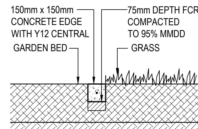
CONCRETE MOWING EDGE DETAIL SCALE 1:40 @ A3
