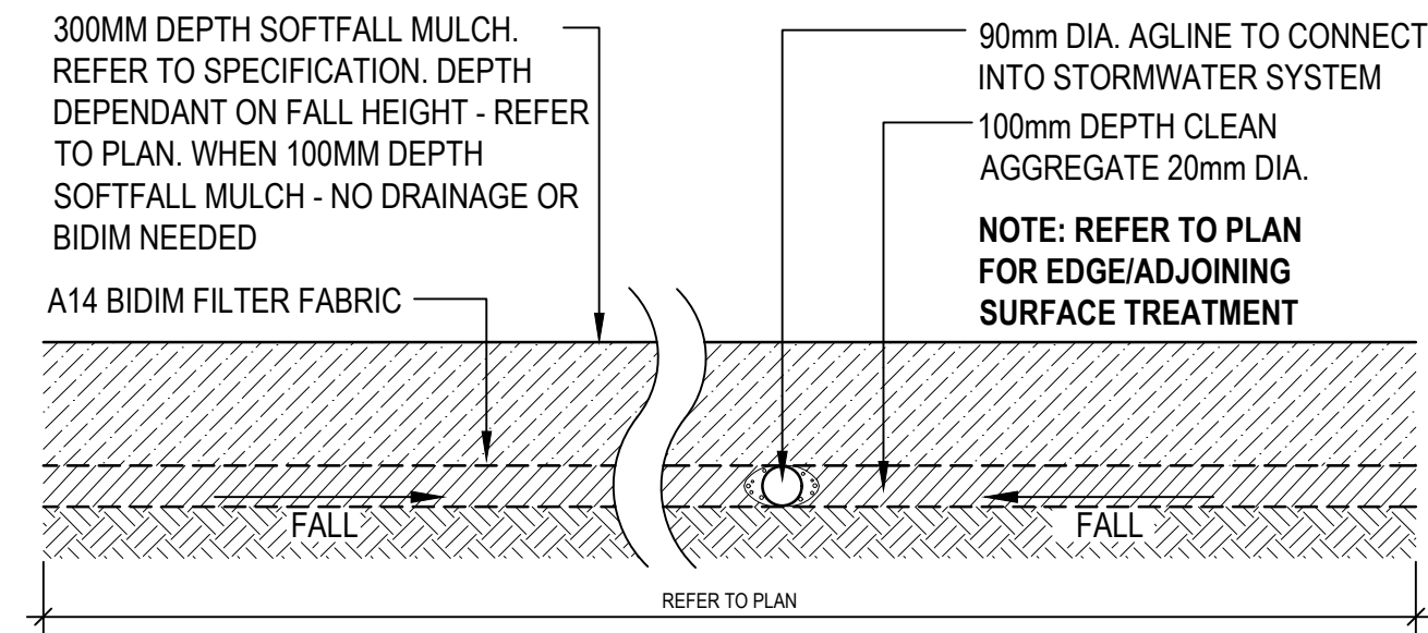
CHILDRENS PLAYGROUND-SOFTFALL MULCH TYPICAL SECTION SCALE 1:40 @A3
